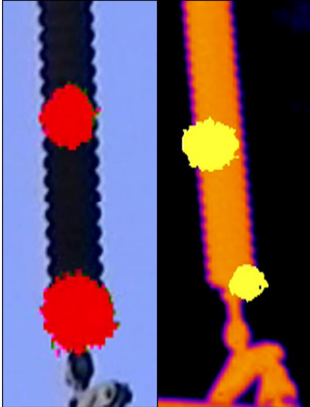
Corona at 2 locations 2 Different causes
