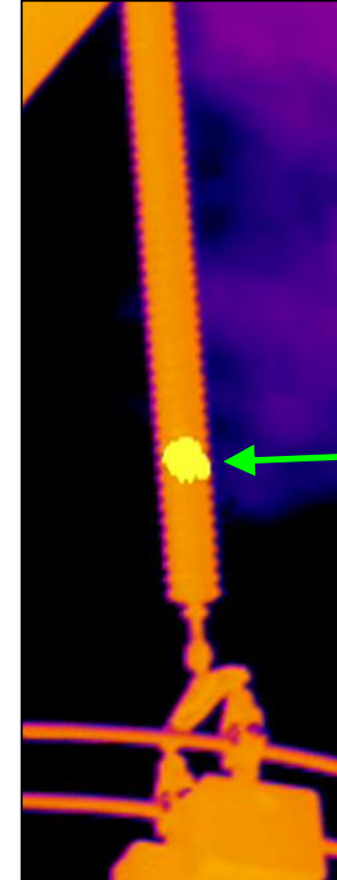
Corona co-located with a hotspot indicating internal tracking – failure within 0-2 years*
