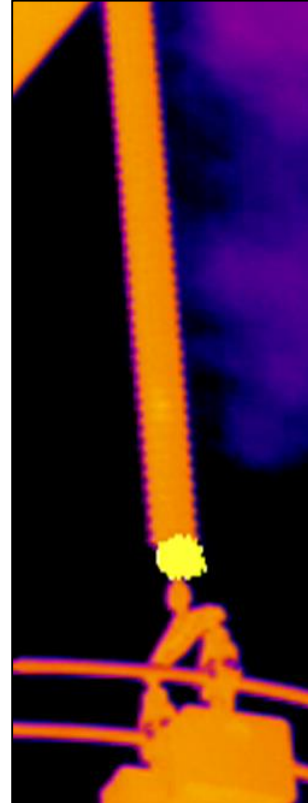
End Fitting Corona – failure within 4-10 years*
