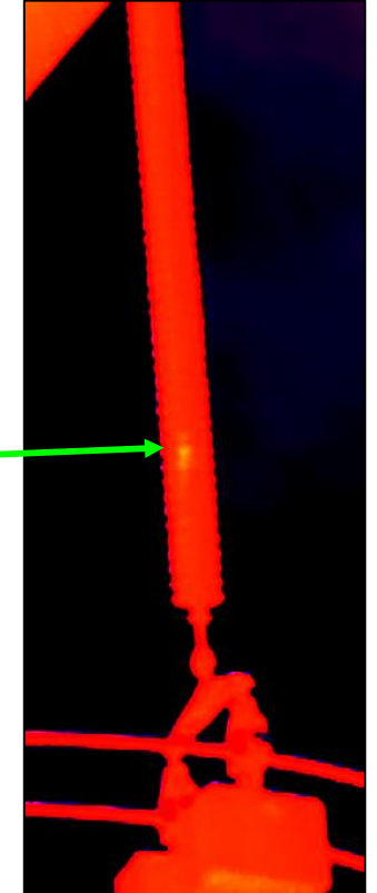
Corona co-located with a hotspot indicating internal tracking – failure within 0-2 years*
