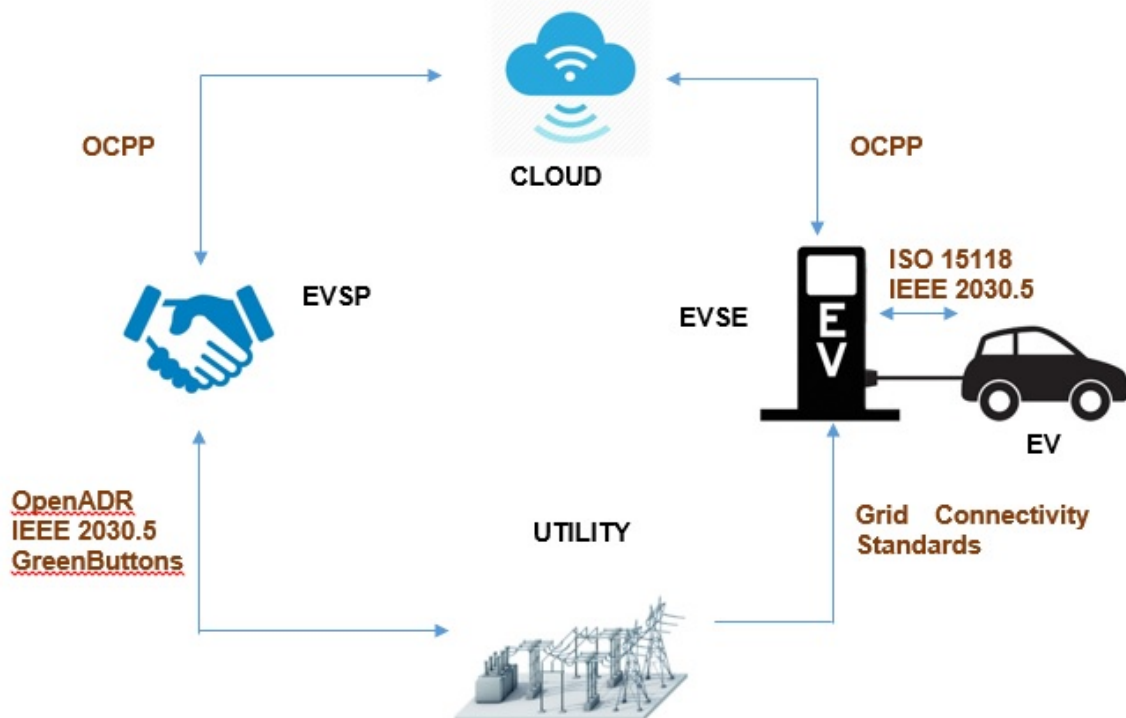
Figure 13: EVSE Communication Protocol
