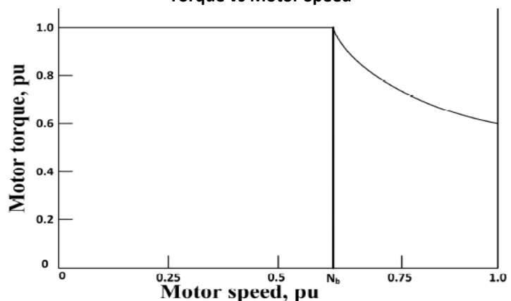
Figure 18: Permanent Magnet Brushless DC Motor: Motor Torque vs Motor Speed
