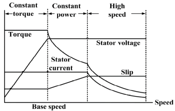
Figure 19 Induction Motor: Motor Torque vs Motor Speed
