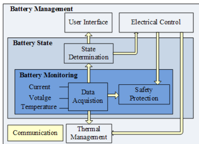
Figure 14: Battery Management System
