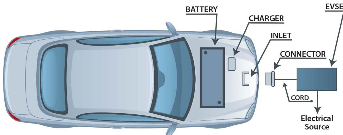
Figure 12: EV Components
