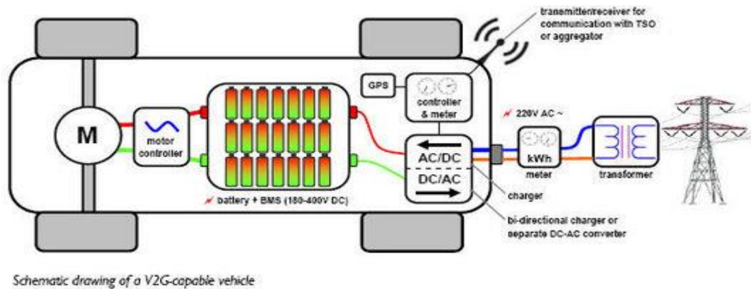
Figure 17: Vehicle to Grid Capable Vehicle
