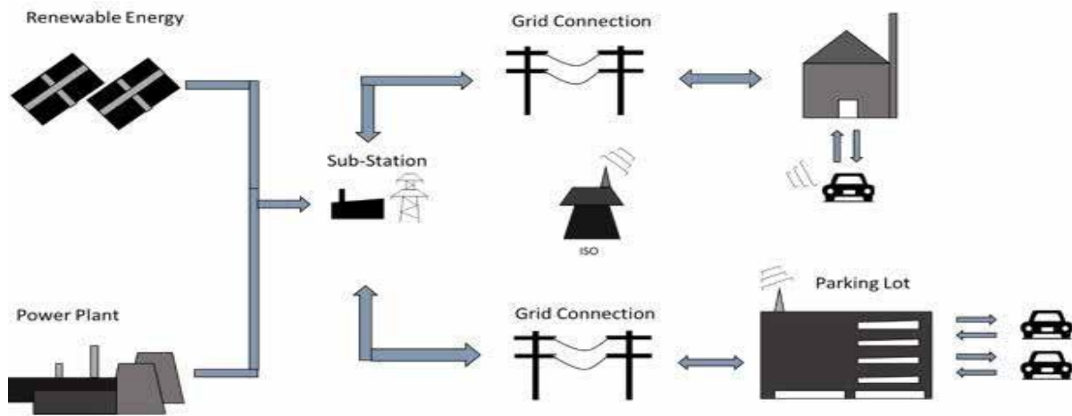
Figure 16: Vehicle to Grid Integration (V2G)
